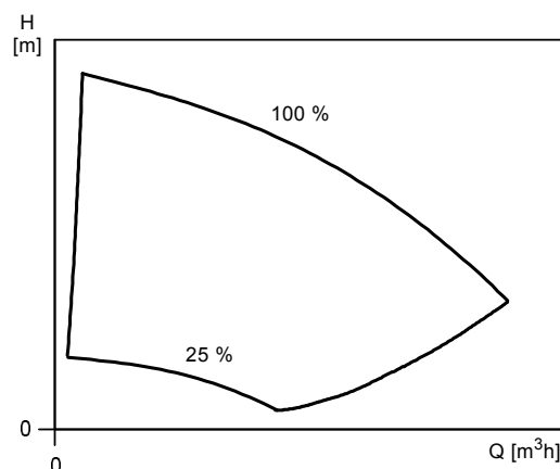
Fig. 13 Duty range of TPE Series 1000 pumps
