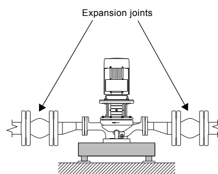
Fig. 86 TP pump installed with larger expansion joints
