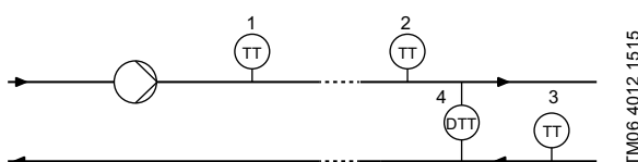
Fig. 56 Overview of Pt100/1000 sensor locations
