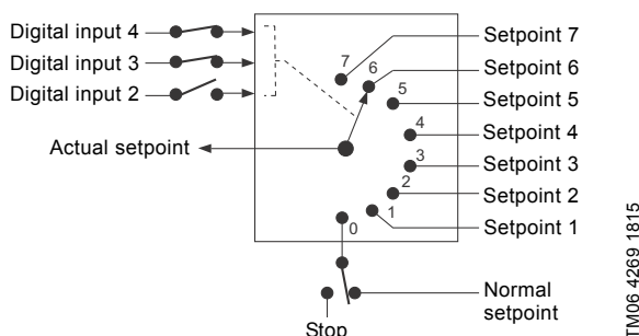
Fig. 66 Principle sketch showing how predefined setpoints function
