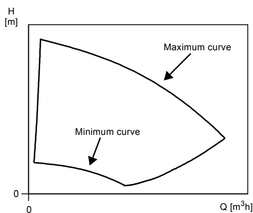
Fig. 73 Minimum and maximum performance curves
