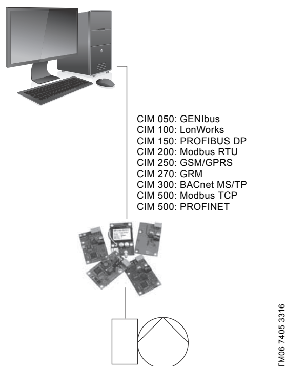
Fig. 72 Structure of a central building management system
