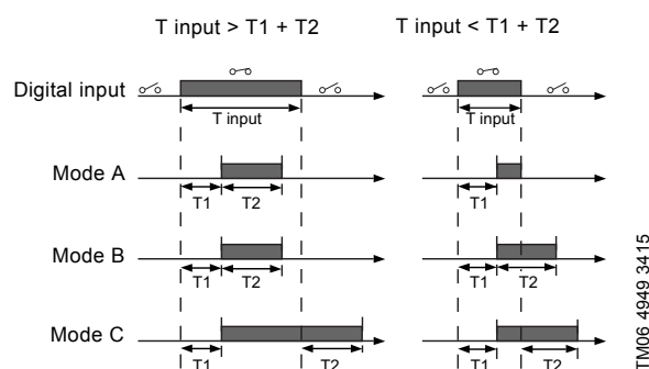
Fig. 59 Duration timer function of digital inputs
