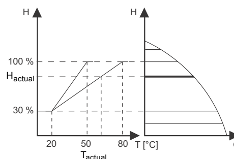
Fig. 67 Temperature influence
