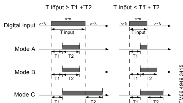
Fig. 57 Duration timer function of digital inputs
