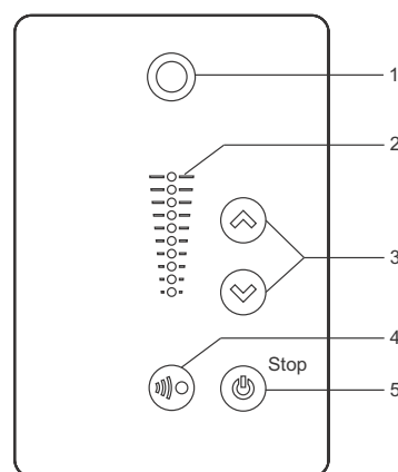
Fig. 21 Standard control panel
