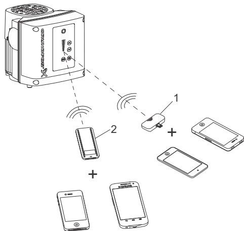
Fig. 33 Grundfos GO communicating with the pump via radio or infrared connection, IR
