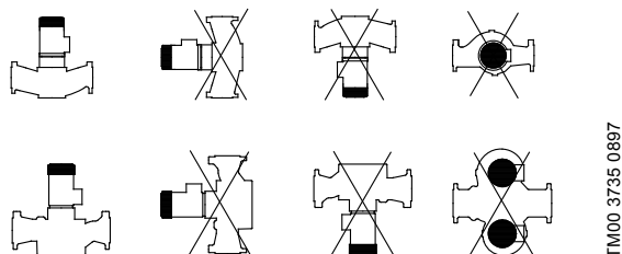
Fig. 78 Installation of motor sizes of 11 kW and up
