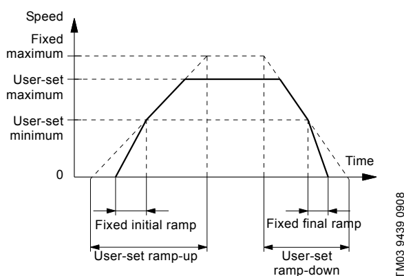
Fig. 69 Ramp-up and ramp-down
