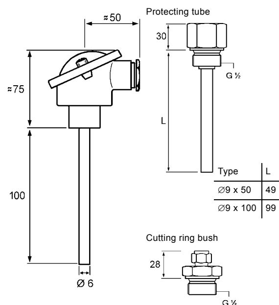
Fig. 99 Dimensional sketch
