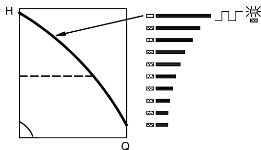
Fig. 29 Maximum curve duty
