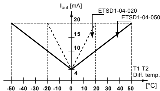
Fig. 100 Sensor characteristics
