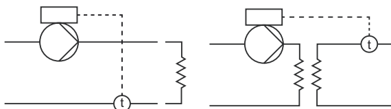
Fig. 43 Constant temperature
