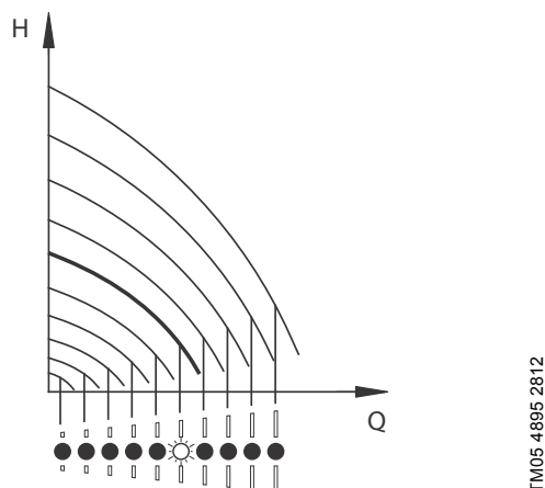
Fig. 23 Pump in constant-curve control mode
