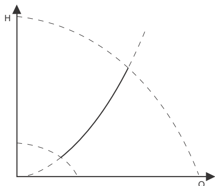
Fig. 50 "Constant level"
