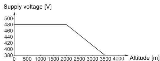
Fig. 4 Supply voltage for three-phase motor in relation to altitude
