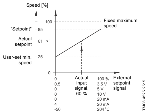
Fig. 62 Example of setpoint influence with constant curve
