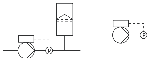
Fig. 41 "Constant pressure"
