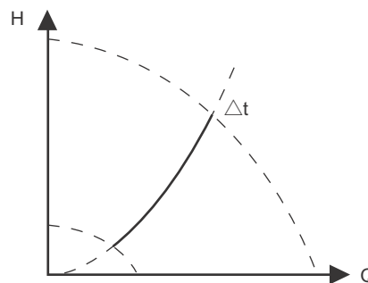
Fig. 46 "Constant differential temperature"
