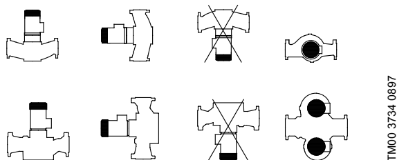
Fig. 77 Installation of motor sizes smaller than 11 kW
