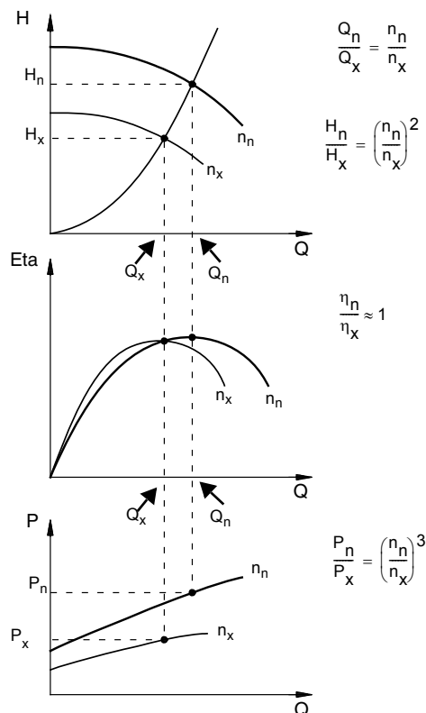
Fig. 74 Affinity equations
