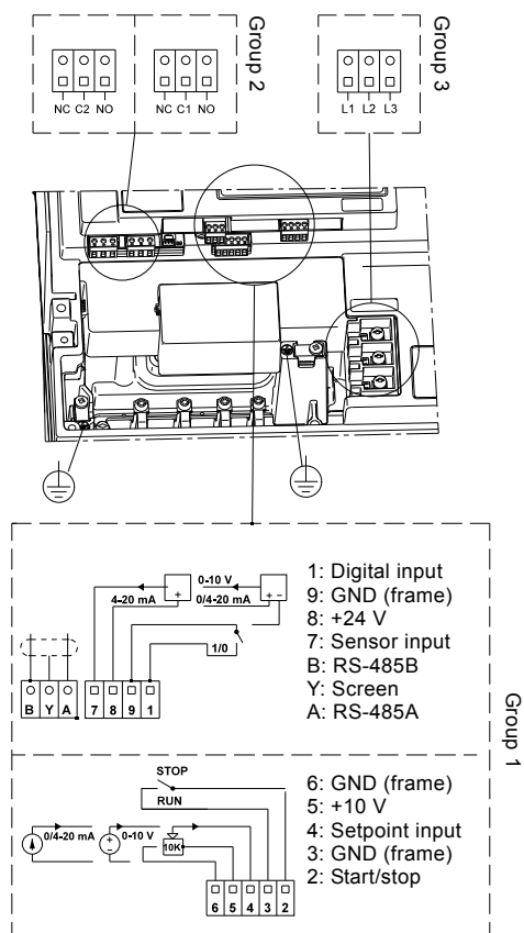
Fig. 94 Connection terminals
