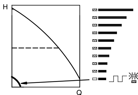
Fig. 30 Minimum curve duty
