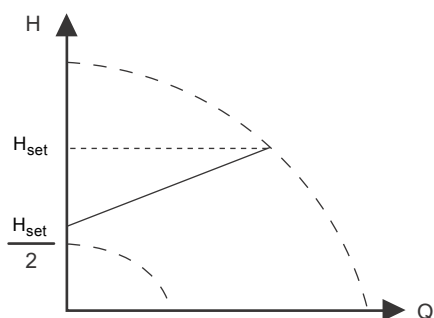
Fig. 38 "Proportional pressure"
