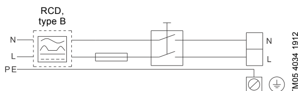
Fig. 90 Example of a mains-connected motor with mains switch, backup fuse and additional protection
