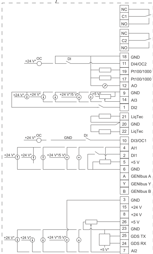
Fig. 92 Connection terminals, FM 300 (option)
